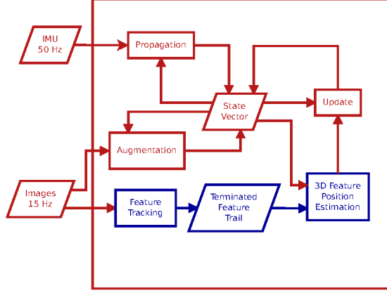
Figure 2. An overview of the 6DOF state estimation algorithm. The state vector appears in Eq. ( 1). The blue-colored components are examined in this paper.
